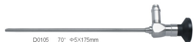
D0105 70° \phi 5 \times 175\text{mm} D0105.1 70° \phi 5 \times 175\text{mm} 134°C 2bar Autoclavable 耐高温高压
