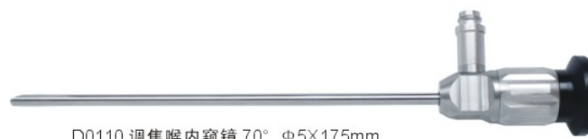
D0110 调焦喉内窥镜 70° \phi 5 \times 175\text{mm} Tele-laryngoscope
