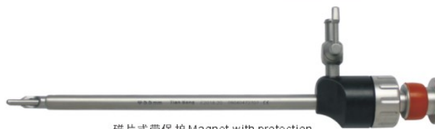
磁片式带保护 Magnet, with protection E2016.20 \Phi 5.5 E2016.21 \Phi 6 E2016.22 \Phi 10.5 E2016.23 \Phi 11
