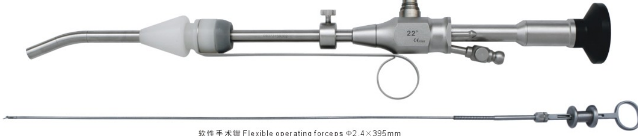
软性手术钳 Flexible operating forceps \Phi 2.4 \times 395\text{mm}
