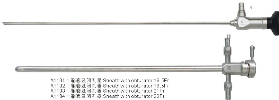
A1105.1 操作器 双通道 Manipulator with two channels
